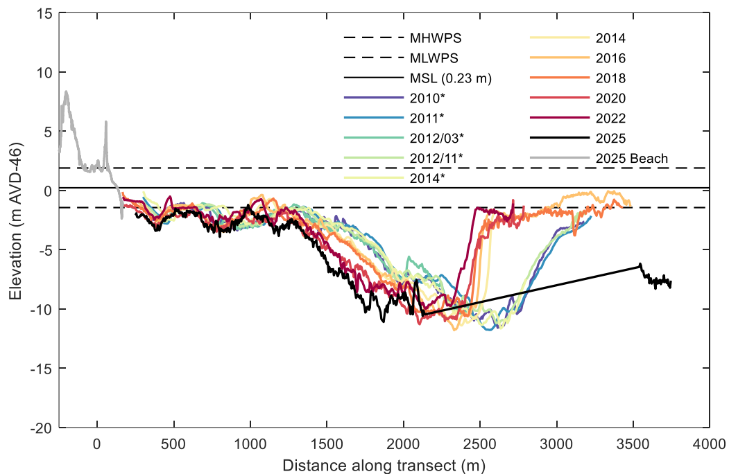
Figure 3-24: Beach and seabed profiles at Transect 5 with comparison to prior surveys on the closely aligned* Transect 3 b . Profile location shown in Figure 2-1 and transect coordinates in Table A-1. *Surveyed on Transect 3 b as approximately parallel to and 200 m south of Transect 5. Straight line in the 2025 profile data is due to the gap illustrated in Figure 2-3.
