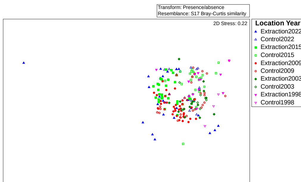
Figure 3-10: Non-metric multidimensional scaling plot (MDS) on presence/absence transformed 9 mm sample data , using Bray Curtis similarities of macrofaunal communities collected from extraction and control sampling sites on Fitzgerald Bank in 1998, 2003, 2009, 2015 and 2022.
