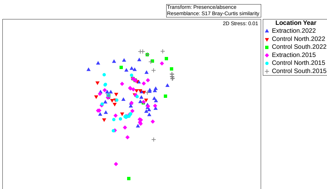
Figure 3-11: Non-metric multidimensional scaling plot (MDS) on presence/absence transformed 1 mm sample data, using Bray Curtis similarities of macrofaunal communities collected from extraction and control sampling sites on Fitzgerald Bank in 2015 and 2022.
