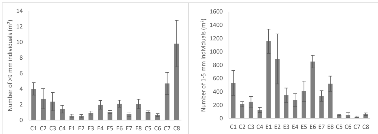
Figure 3-2: Mean density of individuals per m 2 ± standard error per site in the 9 mm sieve (left) and 1 mm sieve (right) in the extraction (E) and control (C) areas.
