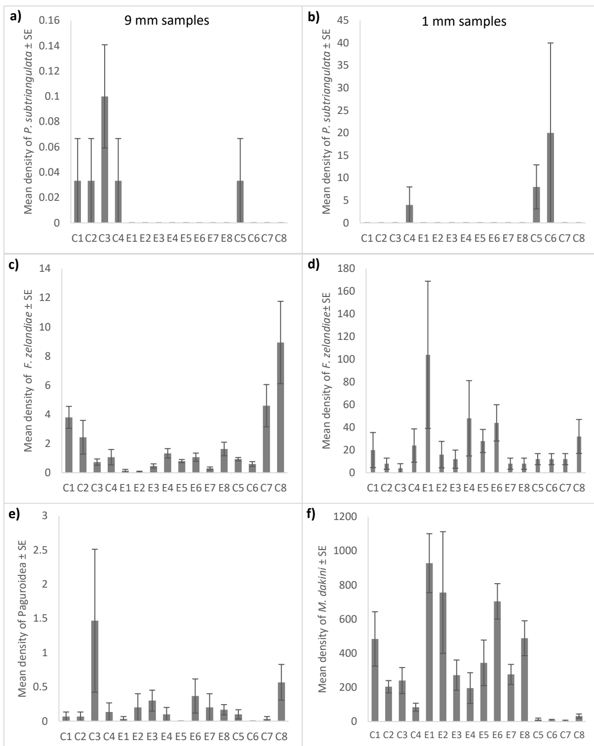
Figure 3-6: Average density of a,b) Paphies subtriangulata , c,d) Fellaster zelandiae , e) Paguroidea and f) Magelona dakini per m 2 ± SE per site (n = 5). Sites designated as extraction (E) and control (C) areas. Left column represents taxa in the 9 mm samples, right represents the 1 mm samples.
