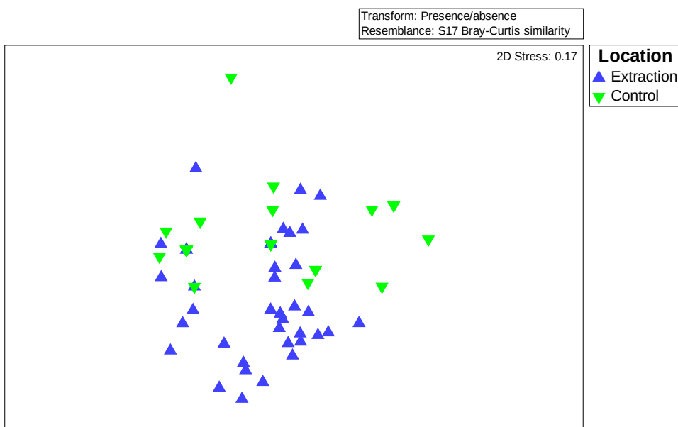
Figure 3-9: Non-metric multidimensional scaling plot (MDS) on presence/absence transformed 2022 1 mm sample data , using Bray Curtis similarities of macrofaunal communities collected from extraction and control sampling areas on Fitzgerald Bank.
