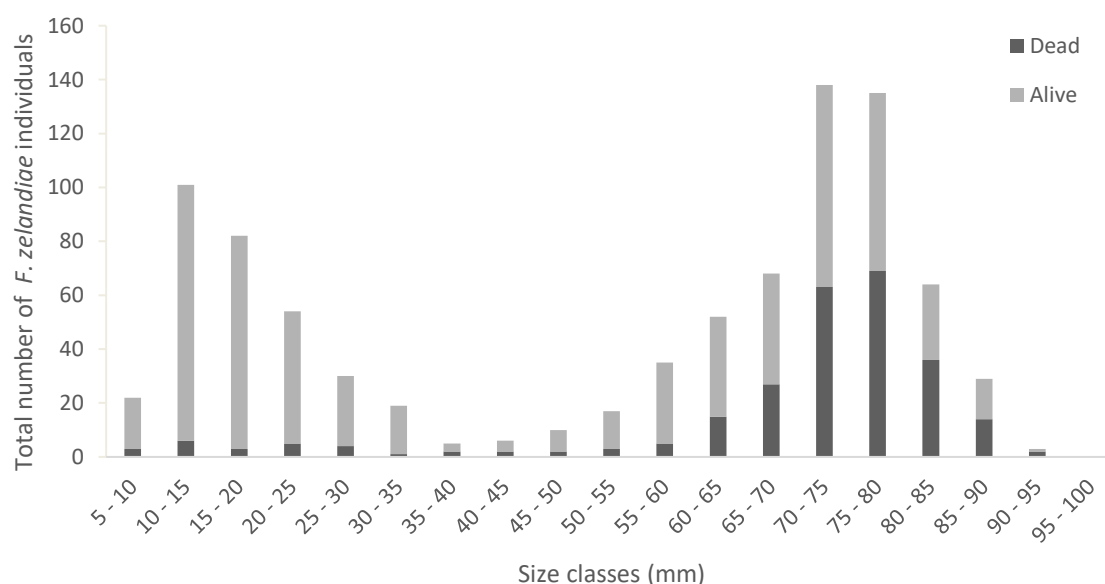
Figure 3-7: Size class distribution of Fellaster zelandiae collected during July 2022 sampling in 1 mm and 9 mm sieves across extraction and control areas combined. Dead represents individuals determined as damaged/not surviving the dredge.
