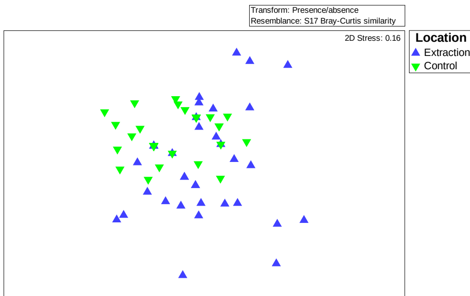
Figure 3-8: Non-metric multidimensional scaling plot (MDS) on presence/absence transformed 2022 9 mm sample data , using Bray Curtis similarities of macrofaunal communities collected from extraction and control sampling areas on Fitzgerald Bank.
