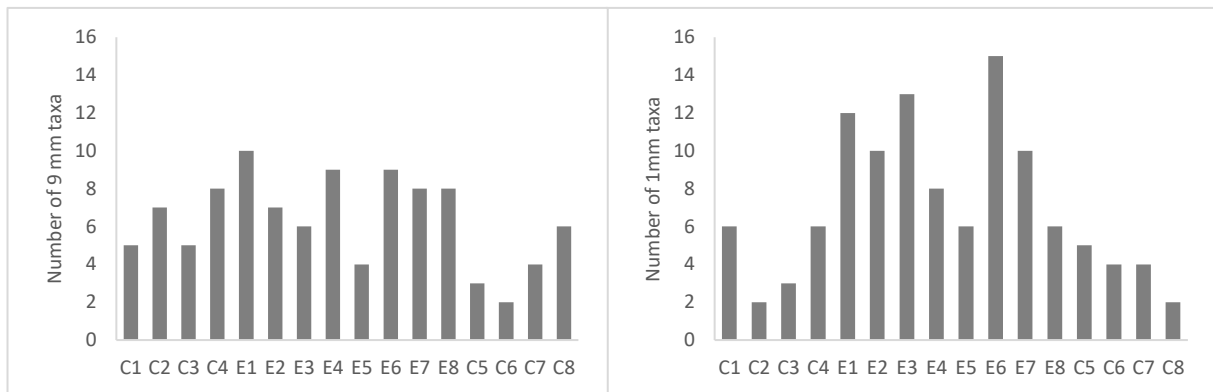
Figure 3-1: Number of taxa present (diversity) per site in the 9 mm sieve from 6 m 2 sample (left) and the 1 mm sieve from 0.05 m 2 sample (right) in the extraction (E) and control (C) areas.
